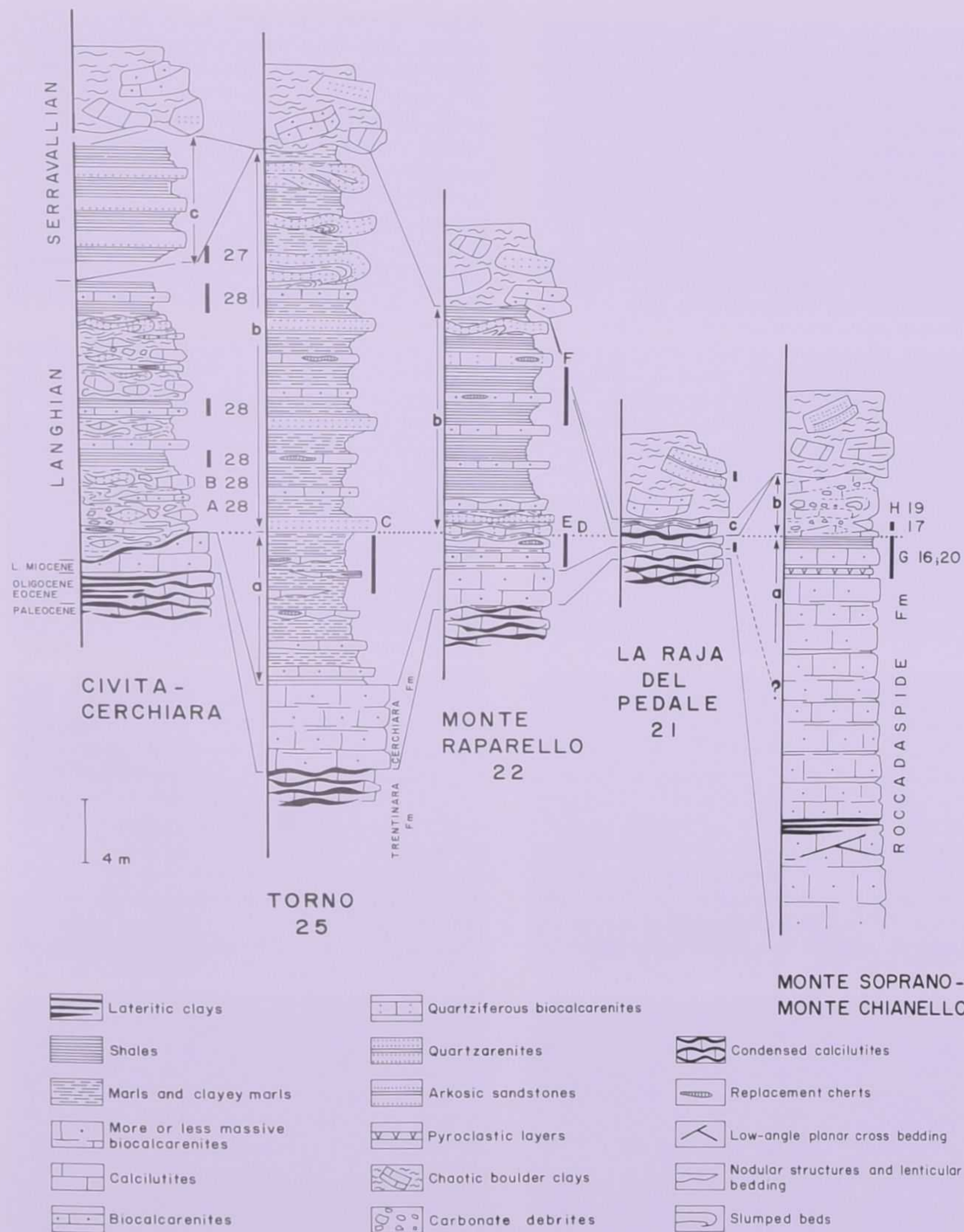
FIG. 7 - Schematic columnar sections representative of the upper part of the Alburno-Cervati carbonate sequence. Symbols (small letters, heavy bars, capital letters and Arabic numerals) have been explained in Fig. 4.
