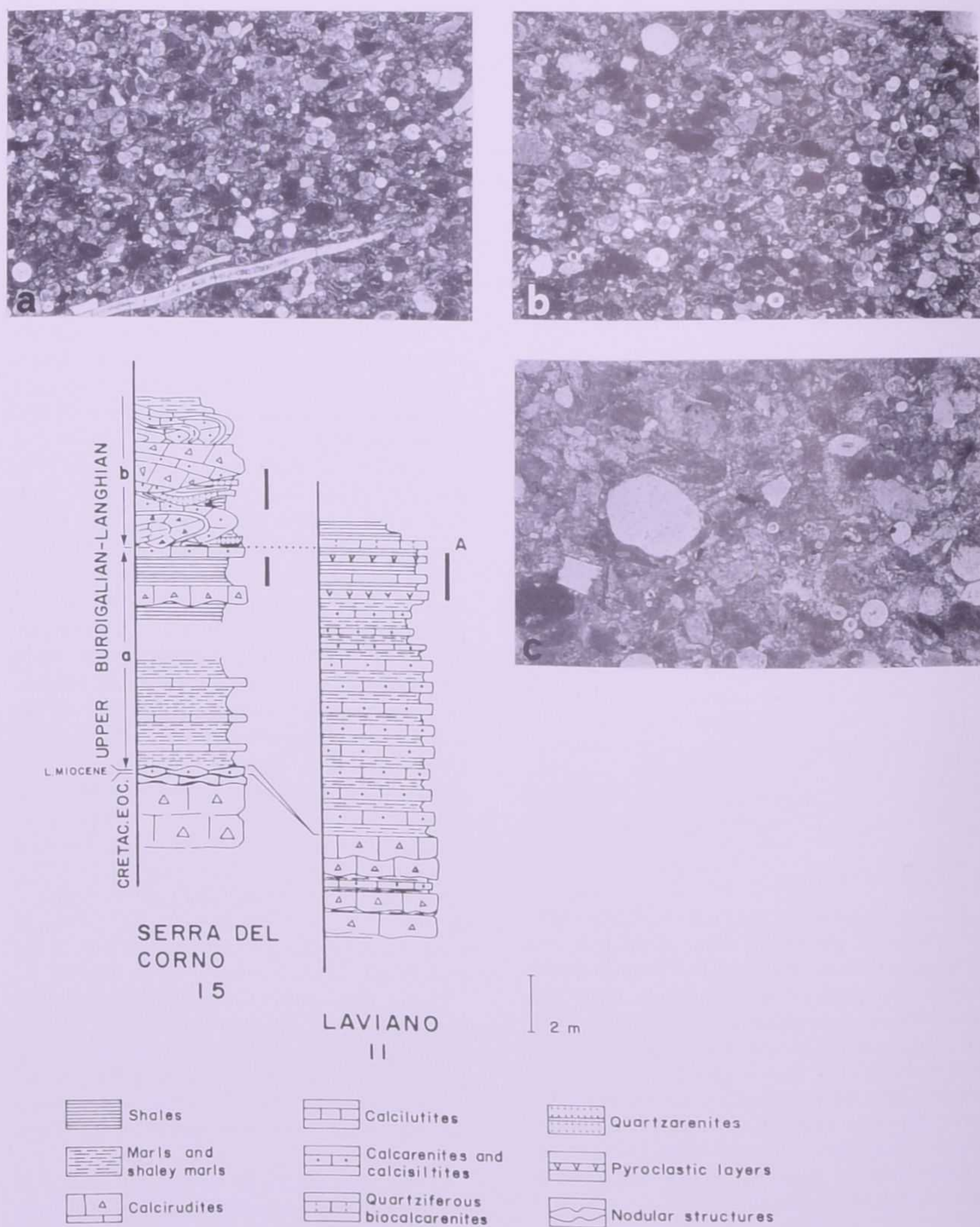
FIG. 10 - Schematic columnar sections of the upper part of the Monti della Maddalena carbonate sequence and examples of microfacies. 10 a - 10 c: spicule-rich packstone with dispersed very fine to fine sand-sized plagioclase (e.g. above the axial section of the spicule in Fig. 10 a) and quartz grains some of them (e.g. Fig. 10 c) well rounded. Laviano, interval b (A position in the columnar section), EP 1621, 10 a and 10 b x 25, 10 c x 63, PPL.
