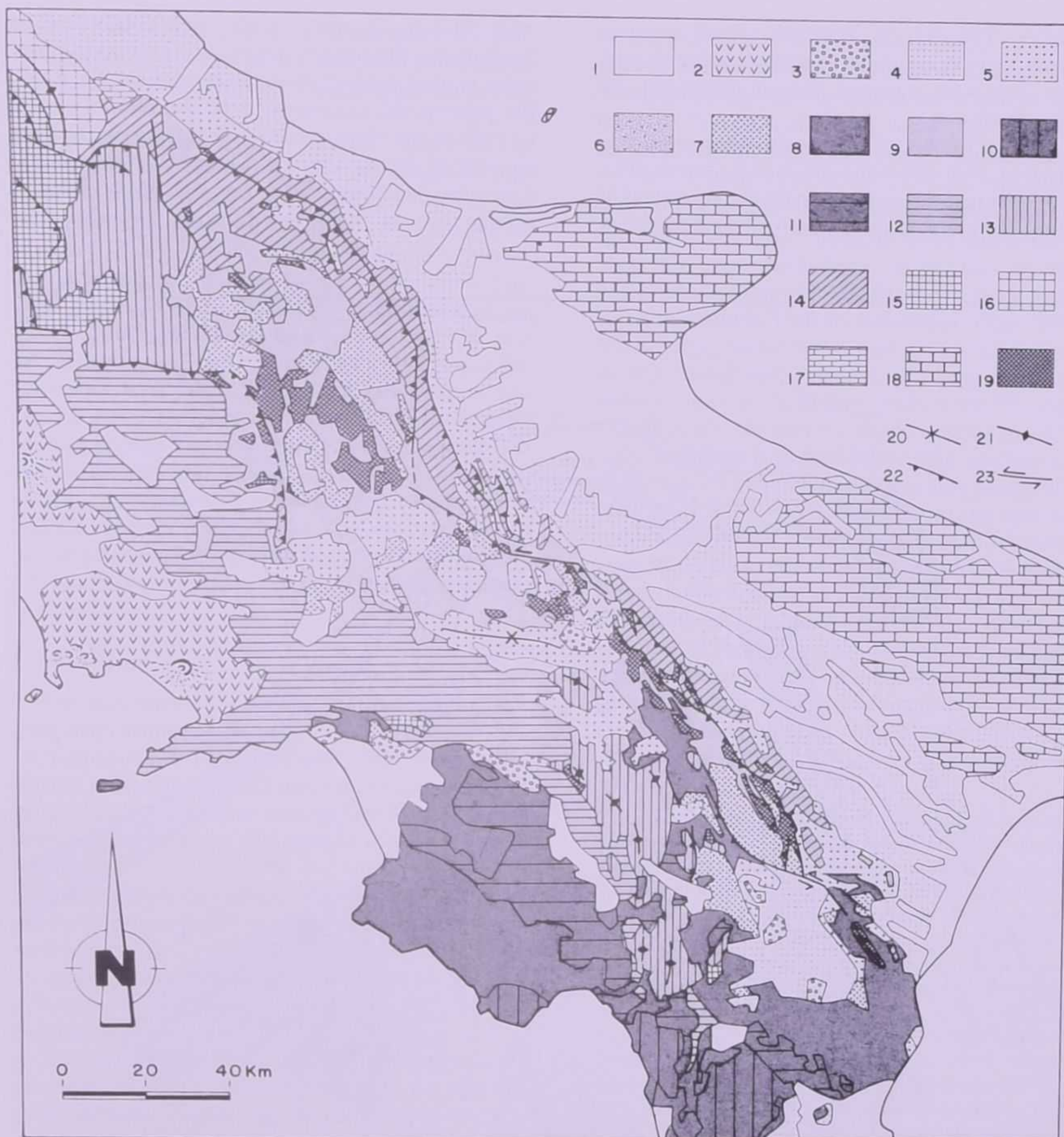
FIG. 1 - Structural sketch of the Southern Apennines and major outcrops of Numidian quartzarenites. 1) continental and subordinate shallow marine deposits ( Holocene-Middle Pleistocene ); 2) volcanites and volcanoclastites ( Holocene-Pleistocene ); 3) lacustrine and fluviolacustrine deposits ( Upper Villafranchian ); 4) Bradano (and Sant' Arcangelo?) sedimentary cycle: shelf-to-continental clastic deposits post-dating the last orogenic transport of the Apennines over the Apulia foreland ( Lower Pleistocene ); 5) Atessa ( Lower Pleistocene p.p. and upper-middle Pliocene ) and Ariano ( middle Pliocene p.p. - lower Pliocene p.p. ) sedimentary cycles: terrigenous shelf deposits unconformably overlying the Apenninic nappes, post-dating the lower Pliocene and the middle Pliocene compression; 6) Branera sedimentary cycle: terrigenous shelf deposits ( lower Pliocene p.p. - Messinian p.p. ) unconformably covering the Apenninic nappes, post-dating the upper Messinian compression; 7) Altavilla, Anzano, Celenza and Gorgoglione sedimentary cycles ( Messinian p.p. - uppermost Tortonian ): siliciclastic deposits, including evaporites and diatomites, post-dating the upper Tortonian compression; 8) internal Apenninic units (Cilento, Sicilide and Calabrian nappes) and Albidona sedimentary cycle; 9) Sannio Nappe; 10) Verbicaro and San Donato units; 11) Alburno-Cervati and Monte Foraporta units; 12) Monti della Maddalena and Matese units, including the Castelvetero and Caiazzo formations; 13) Lagonegro, Frosolone and Agnone units; 14) Tufillo and Daunian units; 15) Scontrone-Porrara Unit; 16) Maiella Unit; 17) Casoli Unit; 18) Mesozoic-Tertiary carbonates of the Apulia foreland; 19) Numidian quartzarenites ( Langhian ); 20) synclines; 21) anticlines; 22) main Pliocene and Pleistocene overthrusts; 23) strike-slip faults.
