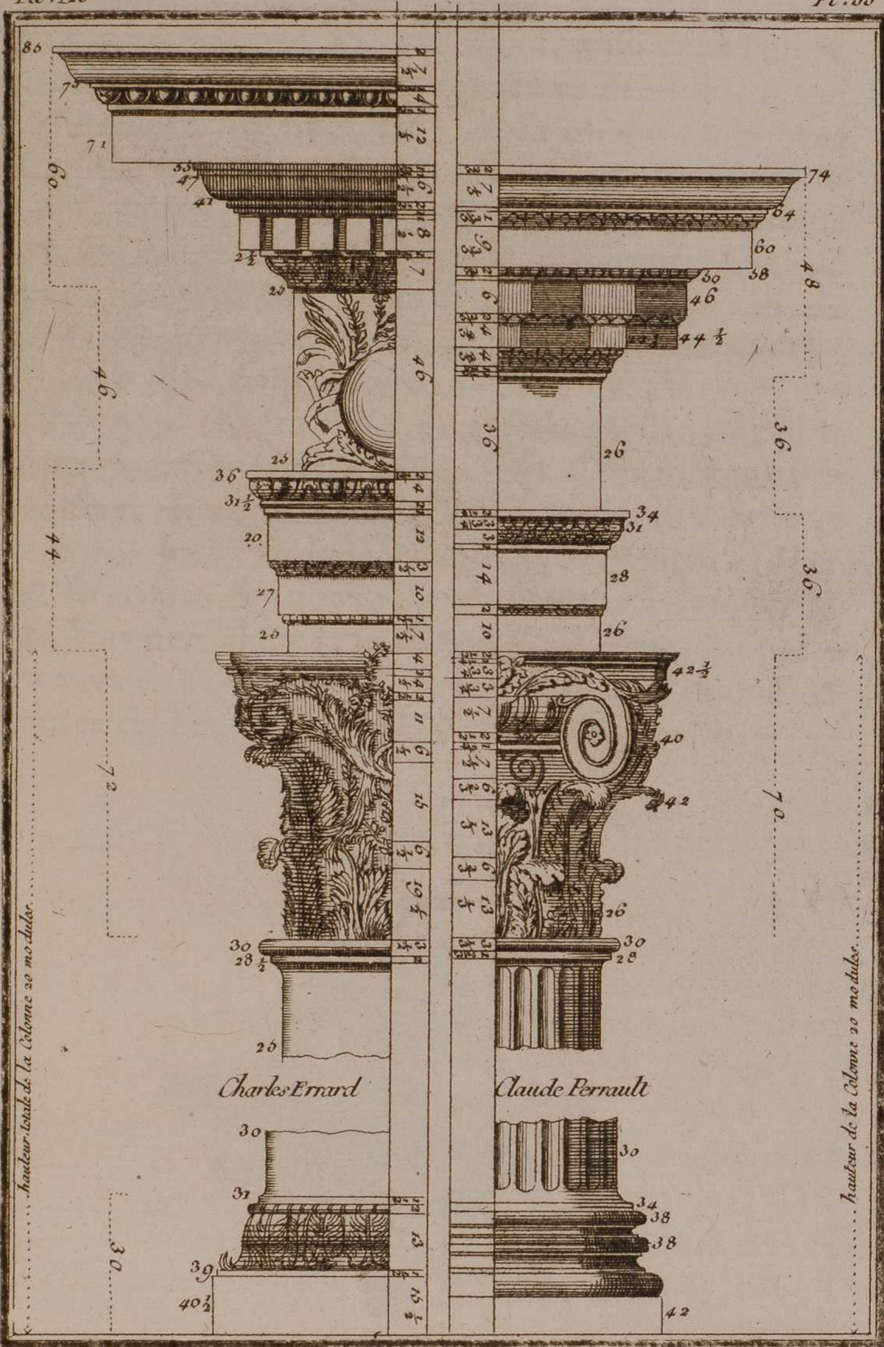
Order Composite
